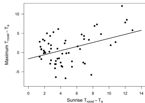
Fig. 4. Positive relationship between maximum T_{\text{roost}}-T_a and sunrise T_{\text{roost}}-T_a for 60 roost days (15 days with 4 available roosts per day) indicating that microclimate conditions at sunrise predict maximum microclimate conditions during the day.
